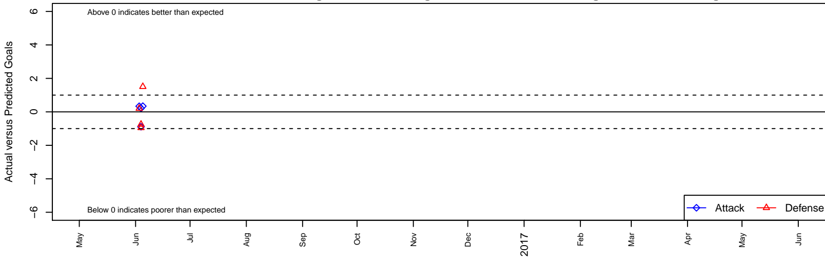
Crossfire Reserves –Unk B99 Dots are actual minus expected GF (blue circles) and GA (red triangles). Blue line is smoothed change in attack strength. Red is smoothed change in defense strength.
